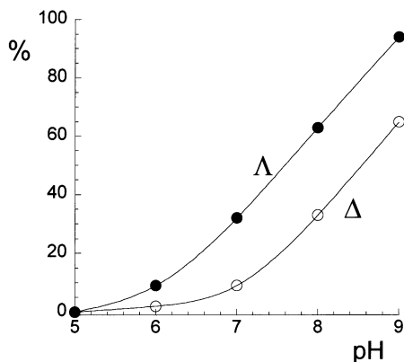
Fig. 2. Amount (%) of electron-transfer mediated fixation of [\text{Co}^{\text{III}}(\text{promp})] to wt azurin as a function of pH. Open circles: \Delta - [\text{Co}((R,R)\text{-promp})] , filled circles: \Lambda - [\text{Co}((S,S)\text{-promp})] . Reaction conditions: [\text{wt-az}] ca. 2 \times 10^{-4} M; [\text{Co}(\text{promp})] = 2 \cdot 10^{-3} M; buffers; 0.1 M; acetate (pH 5.0); MES (pH 6.0); phosphate (pH 7.0); Tris-Cl (pH 8.0); borate (pH 9.0); T = 55^\circ\text{C} .
